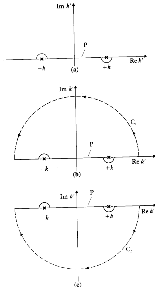
11.4 (a) The path P avoiding the poles at k' = \pm k . (b) Contour ( P + C_1 ) for calculating the integral I_1 . (c) Contour ( P + C_2 ) for calculating the integral I_2 .
